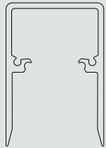
Abdeckprofil rechteckig Cover profile rectangular
